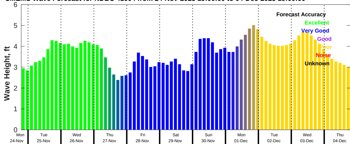
CMEMS Wave Forecast for NDBC 41004 from 24-Nov-2025 19:00:00 to 04-Dec-2025 19:00:00
