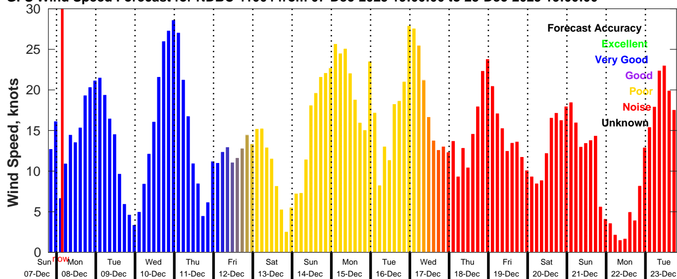
GFS Wind Speed Forecast for NDBC 41004 from 07-Dec-2025 19:00:00 to 23-Dec-2025 19:00:00
