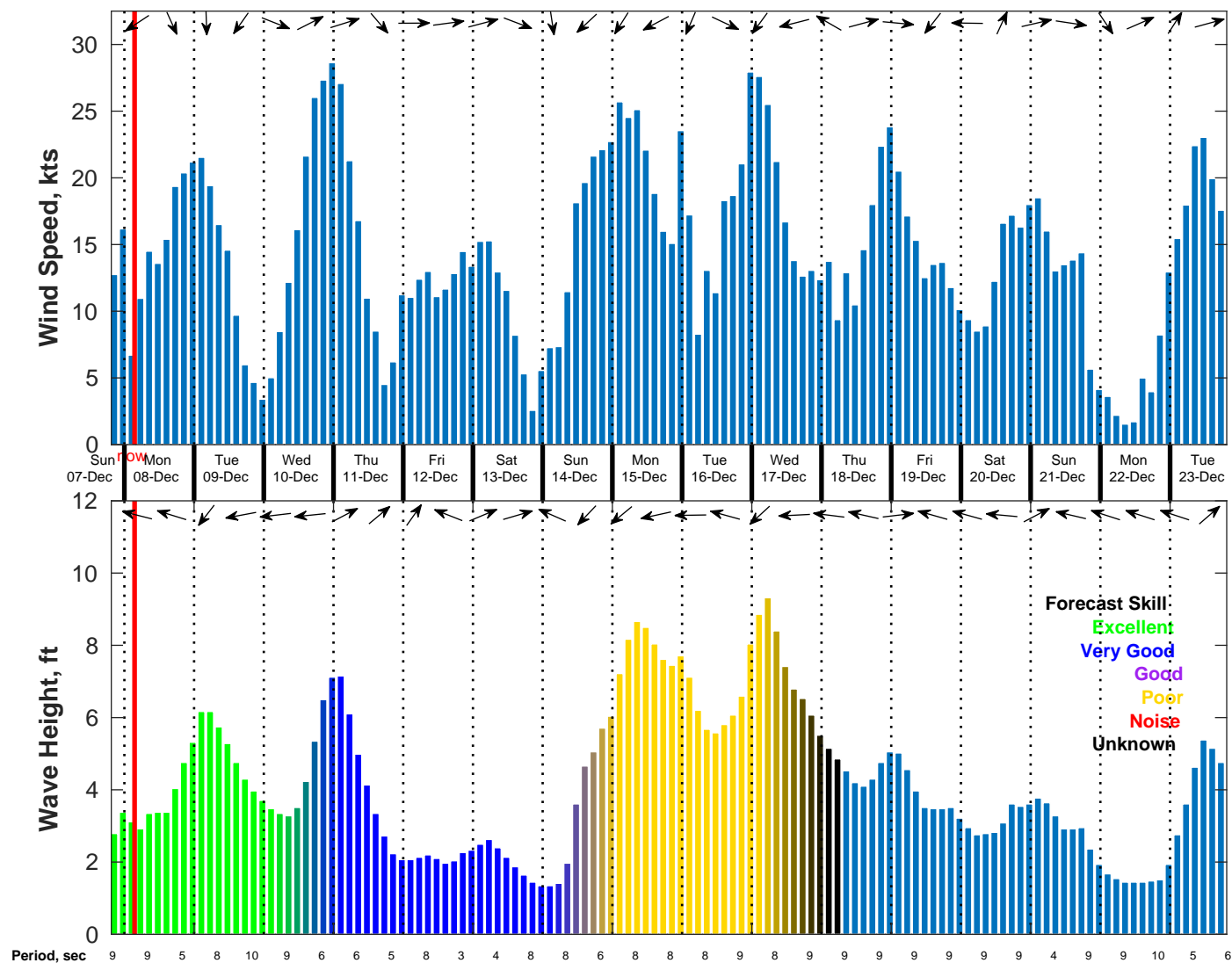
Wind & Wave Forecast for NDBC 41004 from 07-Dec-2025 19:00:00 to 23-Dec-2025 19:00:00
