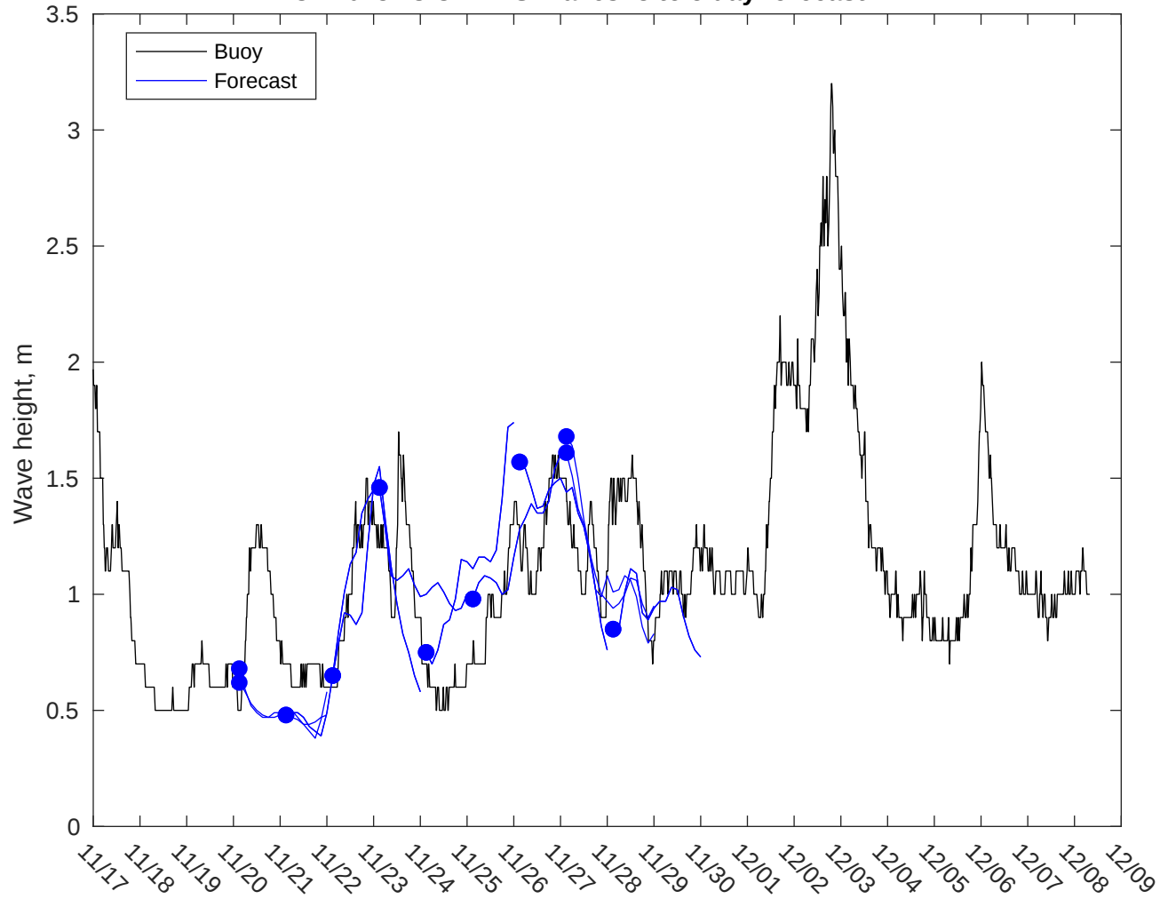
NDBC 41013 vs CMEMS Waves: 3 to 5 day forecast
