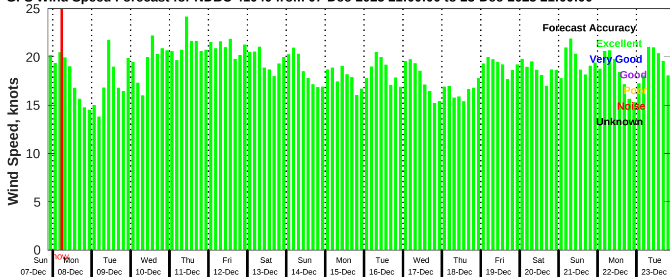
GFS Wind Speed Forecast for NDBC 41040 from 07-Dec-2025 21:00:00 to 23-Dec-2025 21:00:00
