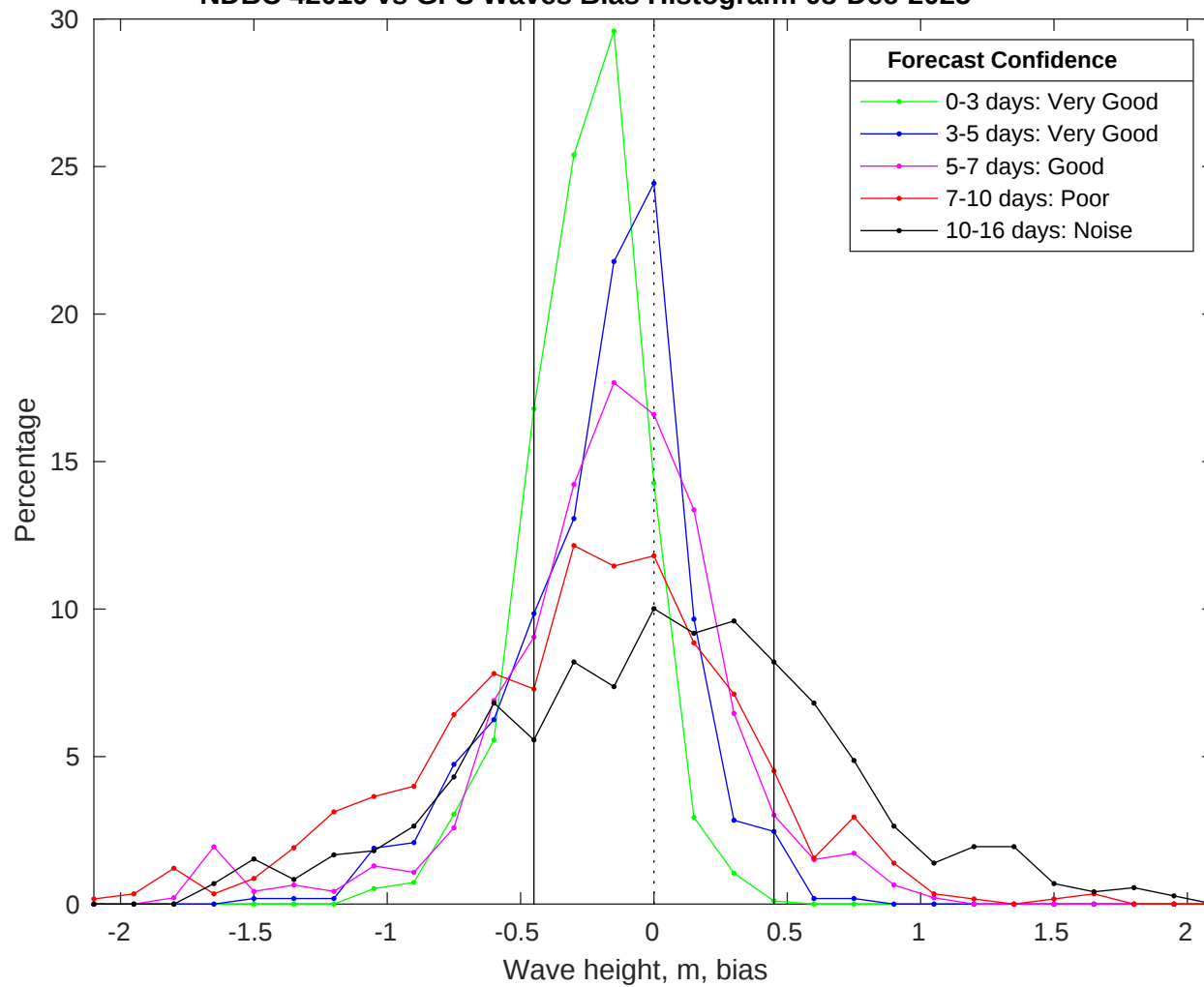
NDBC 42019 vs GFS Waves Bias Histogram: 08-Dec-2025
