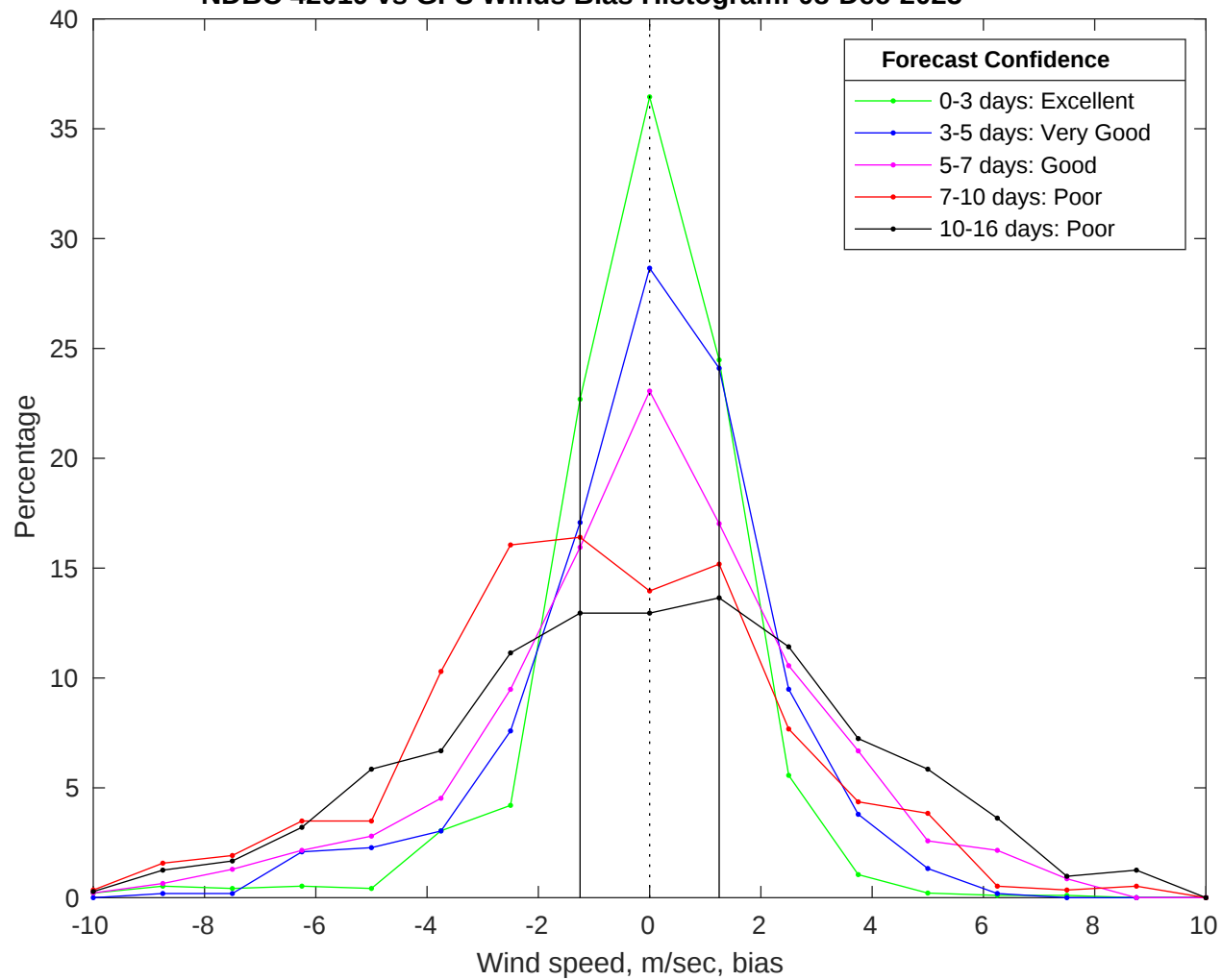
NDBC 42019 vs GFS Winds Bias Histogram: 08-Dec-2025
