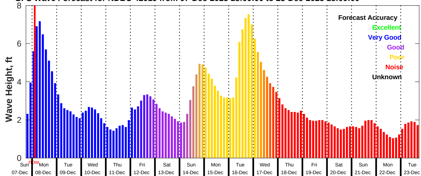
GFS Wave Forecast for NDBC 42019 from 07-Dec-2025 18:00:00 to 23-Dec-2025 18:00:00
