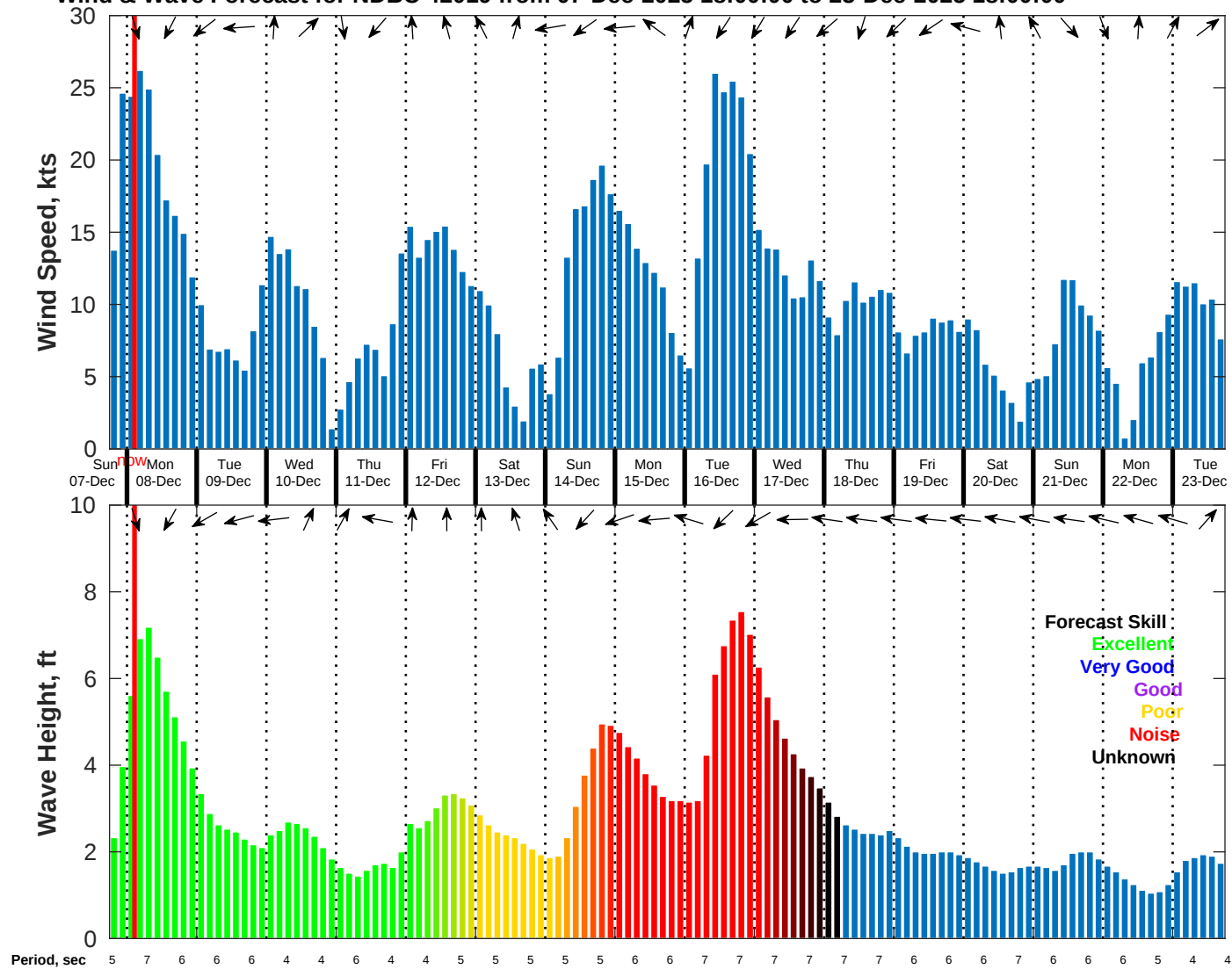
Wind & Wave Forecast for NDBC 42019 from 07-Dec-2025 18:00:00 to 23-Dec-2025 18:00:00
