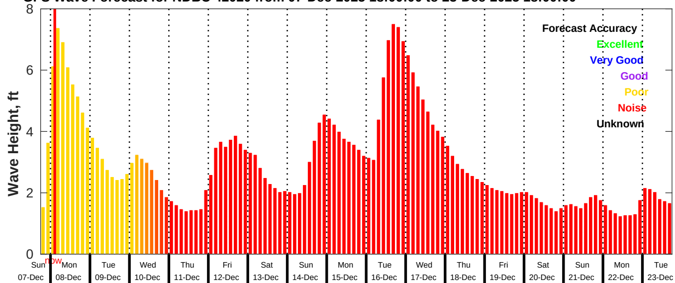
GFS Wave Forecast for NDBC 42020 from 07-Dec-2025 18:00:00 to 23-Dec-2025 18:00:00
