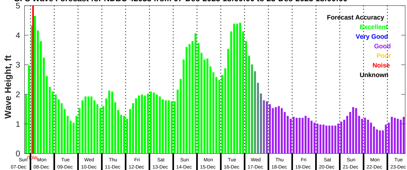
GFS Wave Forecast for NDBC 42035 from 07-Dec-2025 18:00:00 to 23-Dec-2025 18:00:00
