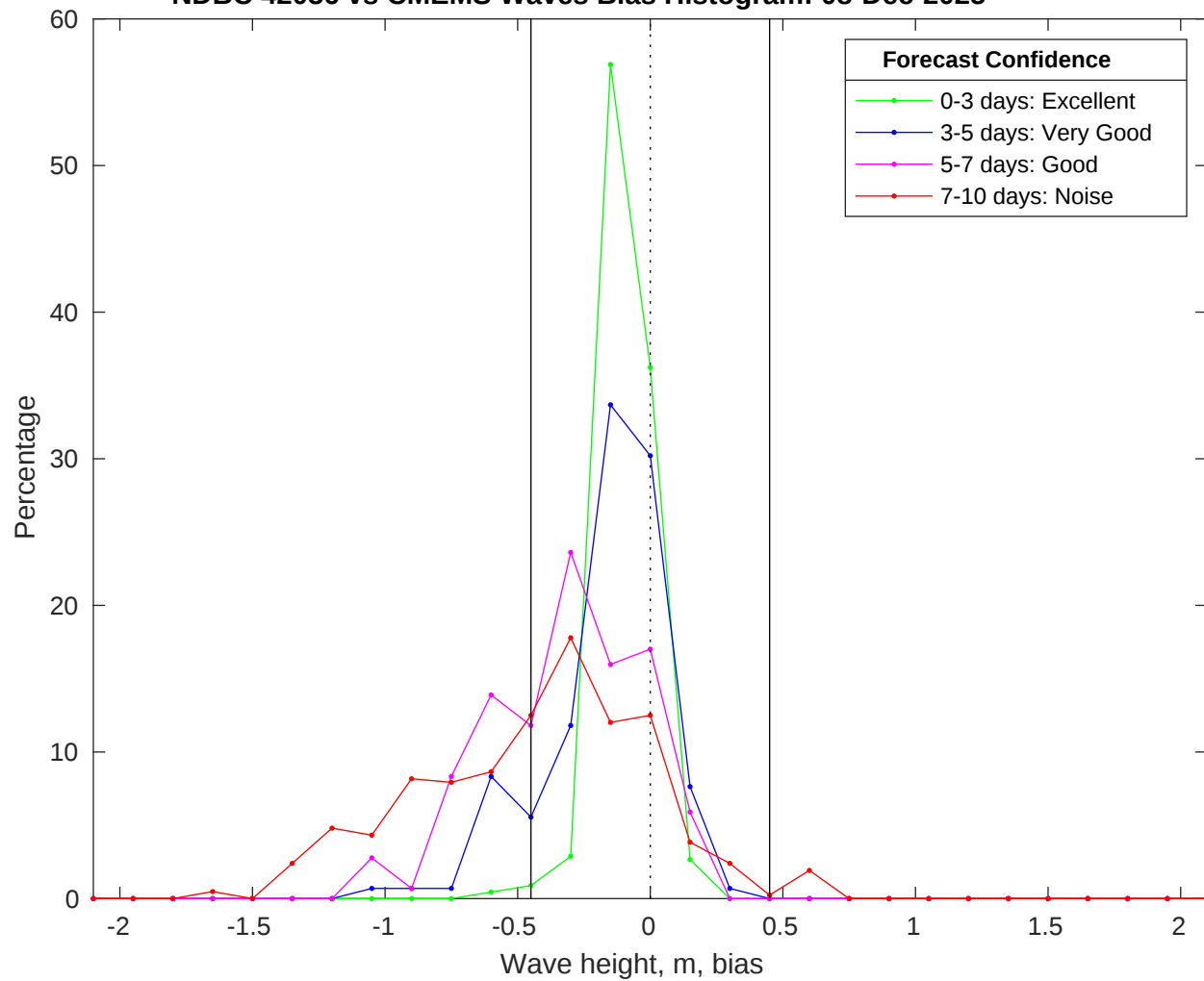
NDBC 42036 vs CMEMS Waves Bias Histogram: 08-Dec-2025
