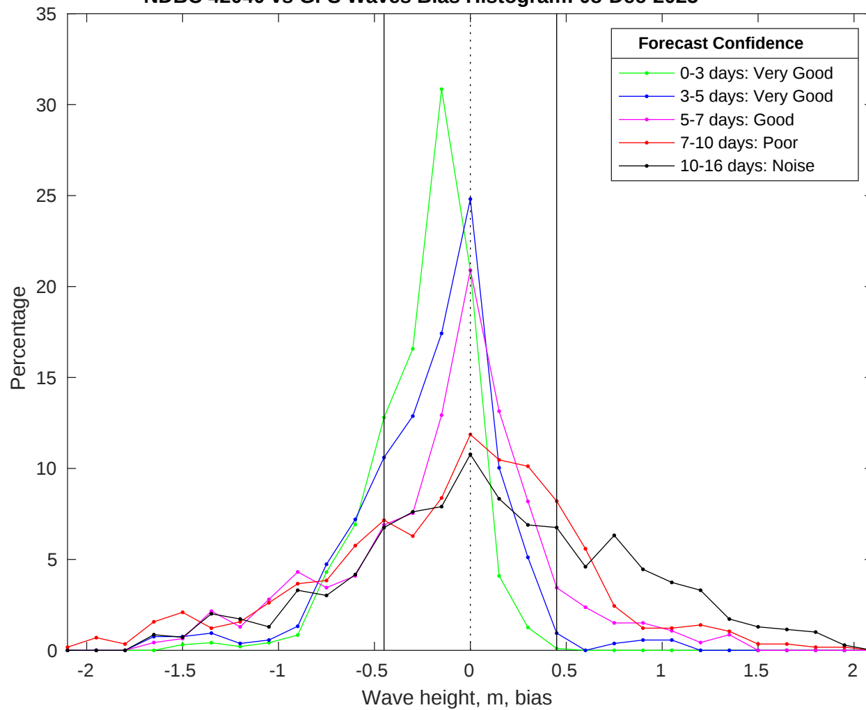
NDBC 42040 vs GFS Waves Bias Histogram: 08-Dec-2025
