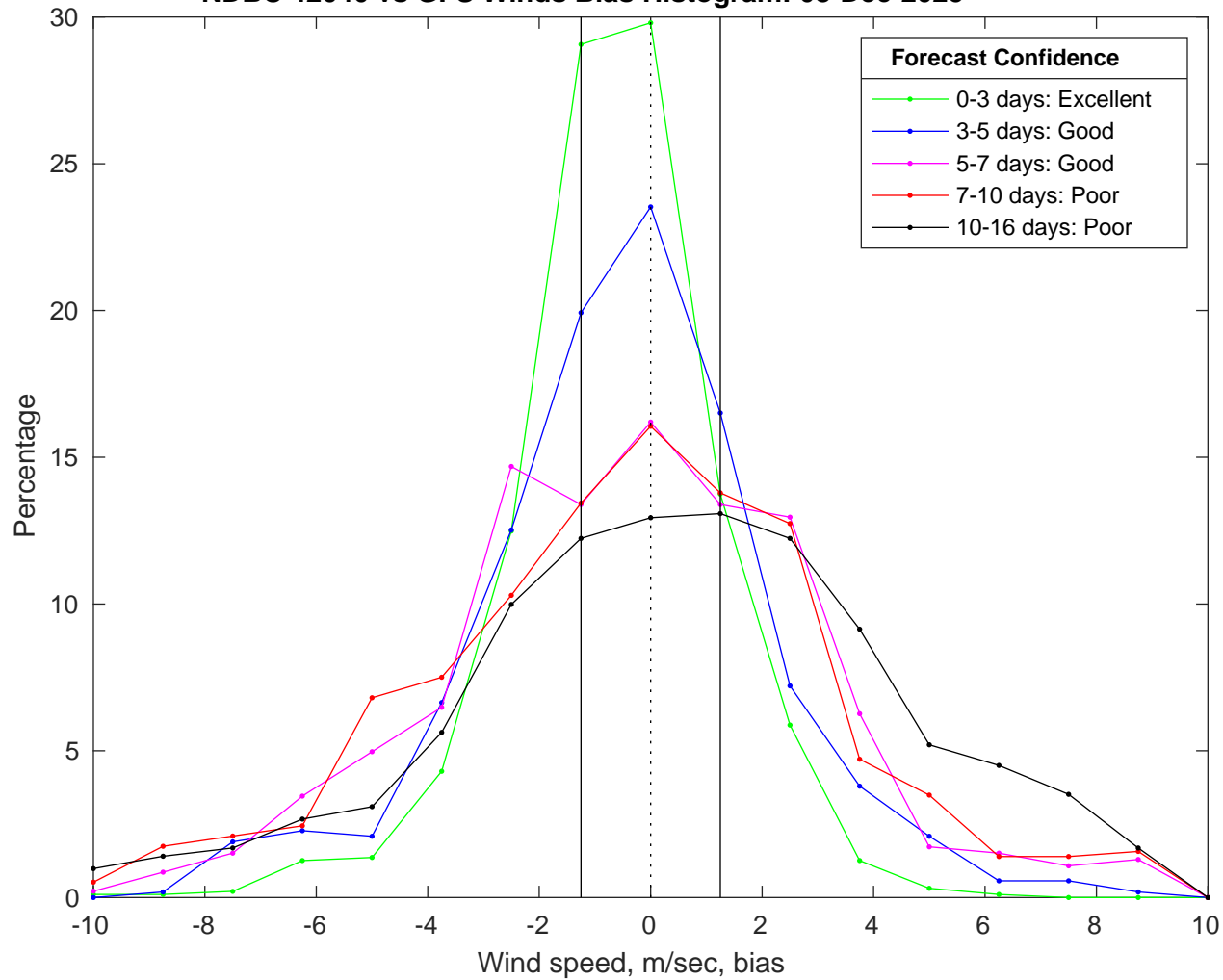
NDBC 42040 vs GFS Winds Bias Histogram: 08-Dec-2025
