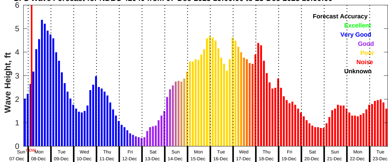
GFS Wave Forecast for NDBC 42040 from 07-Dec-2025 19:00:00 to 23-Dec-2025 19:00:00
