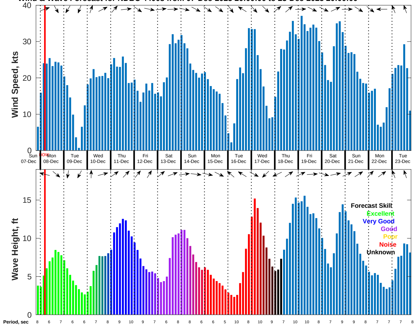
Wind & Wave Forecast for NDBC 44008 from 07-Dec-2025 20:00:00 to 23-Dec-2025 20:00:00
