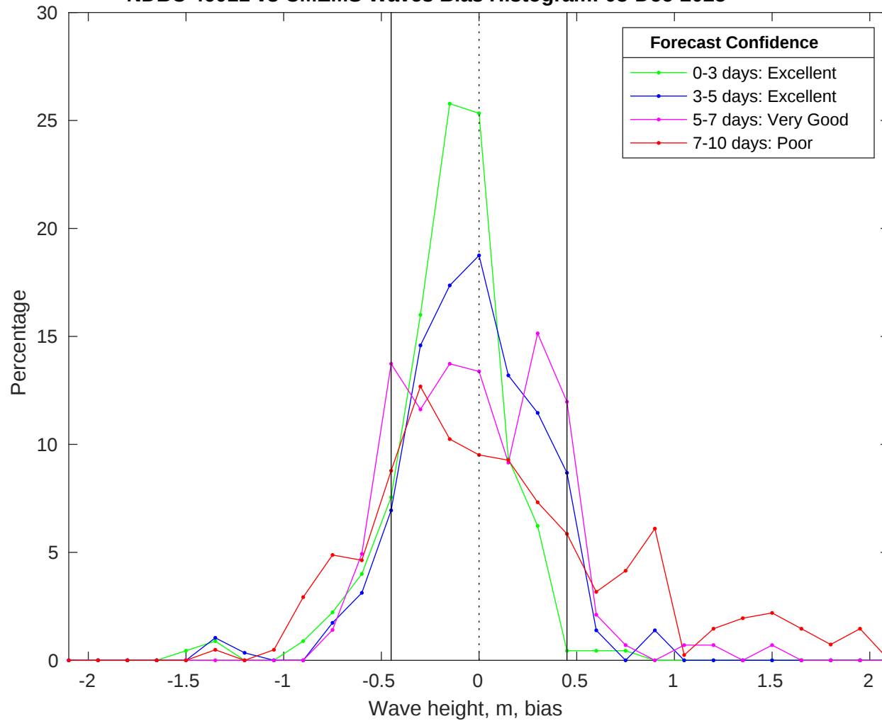
NDBC 46011 vs CMEMS Waves Bias Histogram: 08-Dec-2025
