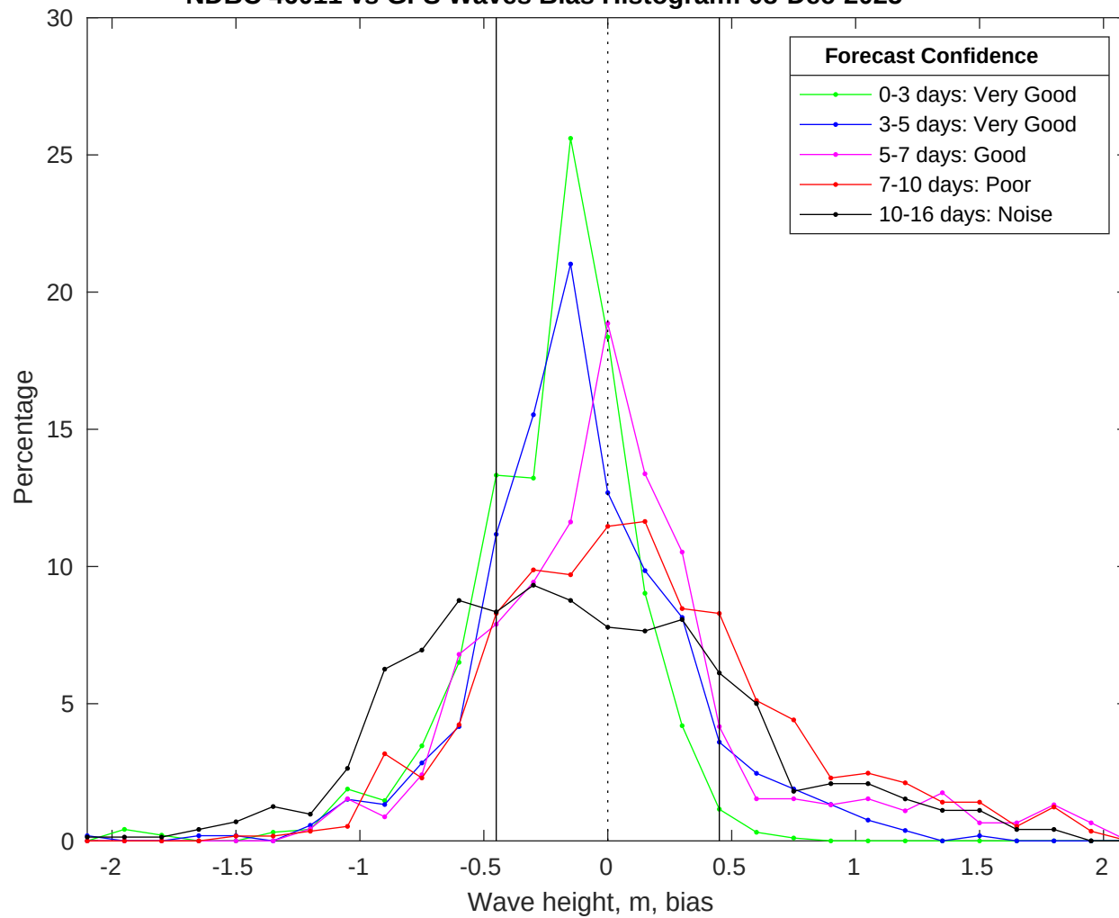
NDBC 46011 vs GFS Waves Bias Histogram: 08-Dec-2025
