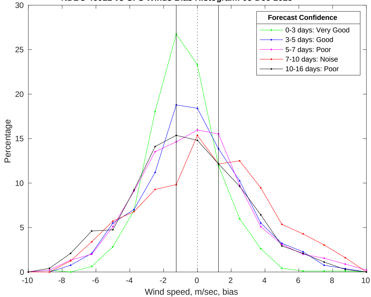
NDBC 46011 vs GFS Winds Bias Histogram: 08-Dec-2025
