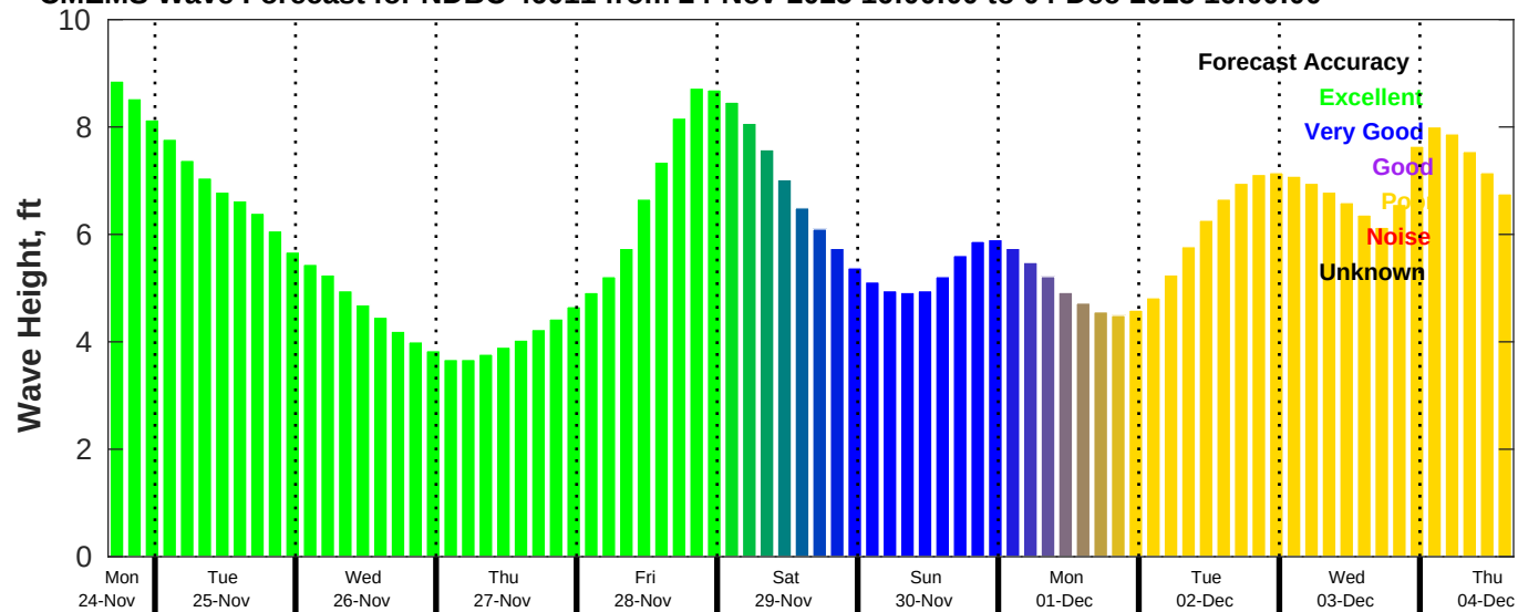
CMEMS Wave Forecast for NDBC 46011 from 24-Nov-2025 16:00:00 to 04-Dec-2025 16:00:00
