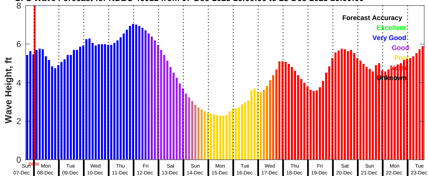
GFS Wave Forecast for NDBC 46011 from 07-Dec-2025 16:00:00 to 23-Dec-2025 16:00:00
