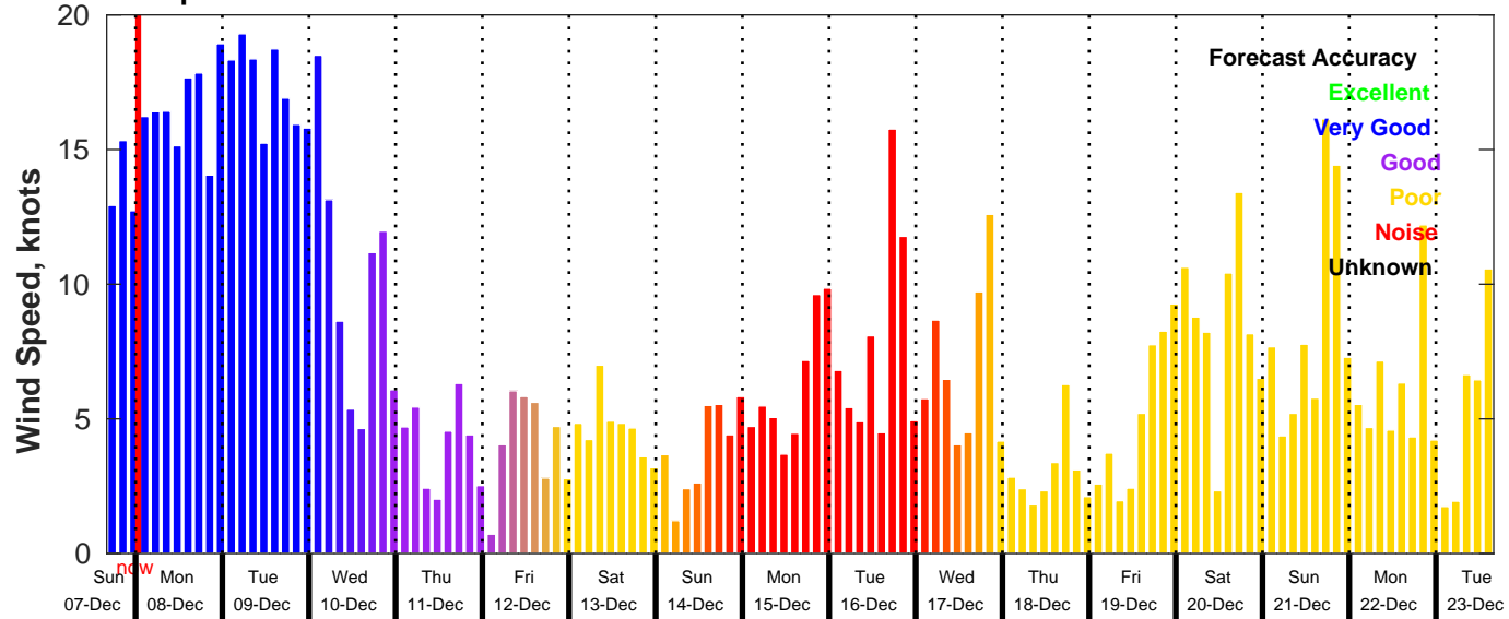
GFS Wind Speed Forecast for NDBC 46011 from 07-Dec-2025 16:00:00 to 23-Dec-2025 16:00:00
