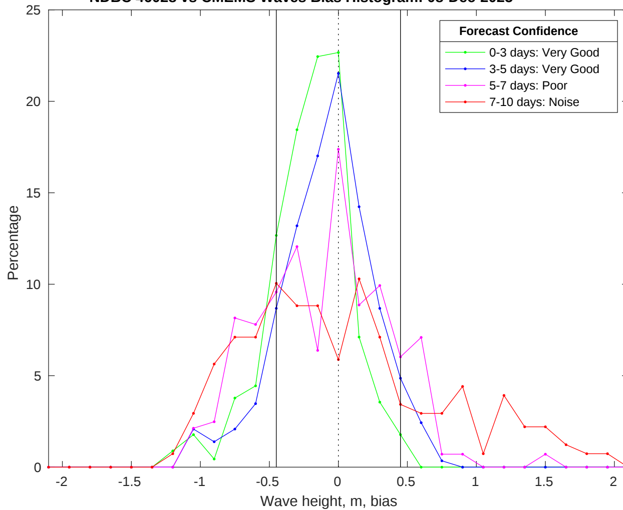
NDBC 46028 vs CMEMS Waves Bias Histogram: 08-Dec-2025
