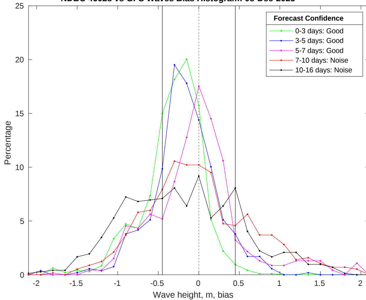
NDBC 46028 vs GFS Waves Bias Histogram: 08-Dec-2025
