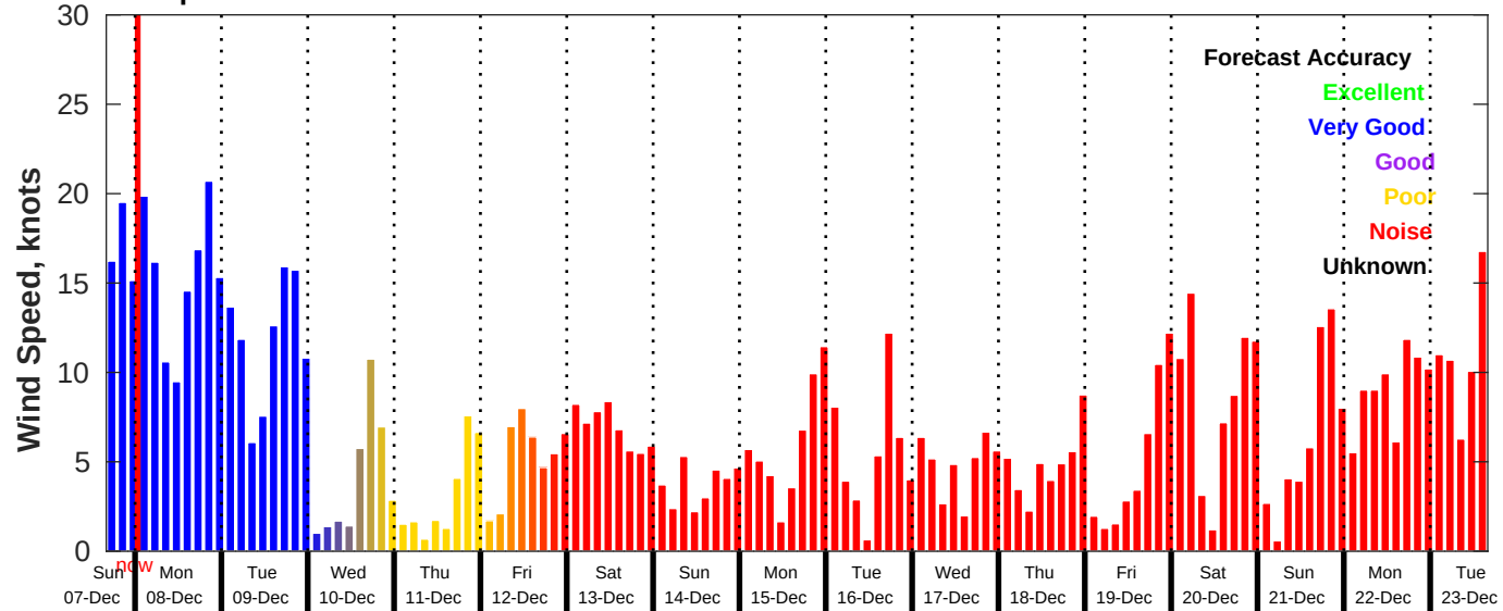
GFS Wind Speed Forecast for NDBC 46028 from 07-Dec-2025 16:00:00 to 23-Dec-2025 16:00:00
