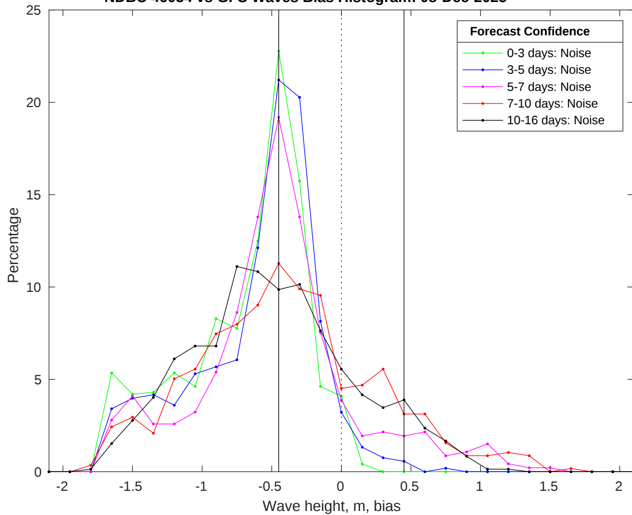
NDBC 46054 vs GFS Waves Bias Histogram: 08-Dec-2025
