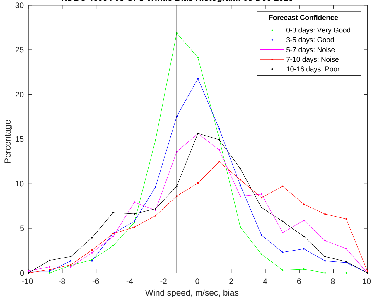
NDBC 46054 vs GFS Winds Bias Histogram: 08-Dec-2025
