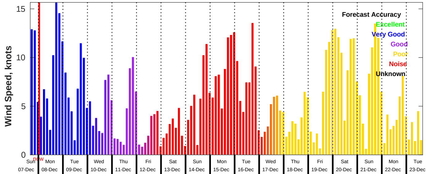
GFS Wind Speed Forecast for NDBC 46054 from 07-Dec-2025 16:00:00 to 23-Dec-2025 16:00:00
