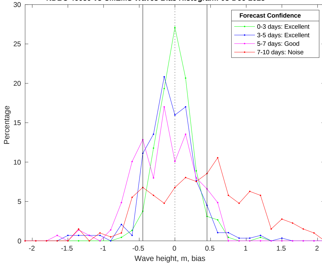
NDBC 46059 vs CMEMS Waves Bias Histogram: 08-Dec-2025
