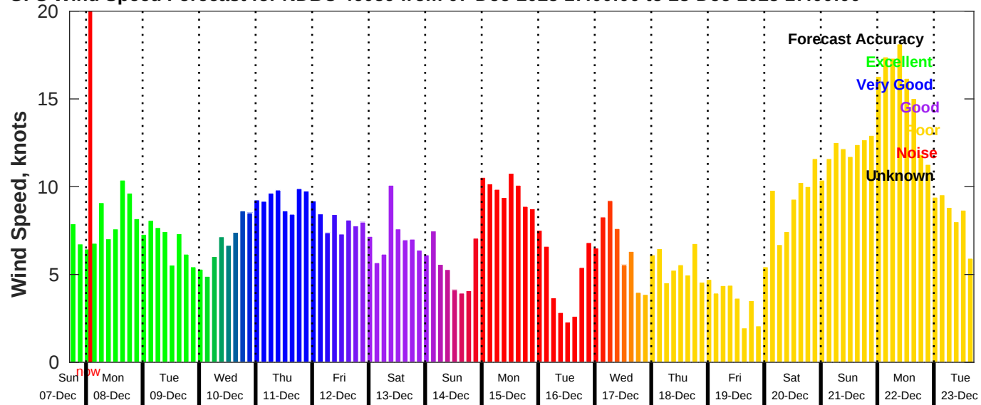
GFS Wind Speed Forecast for NDBC 46059 from 07-Dec-2025 17:00:00 to 23-Dec-2025 17:00:00
