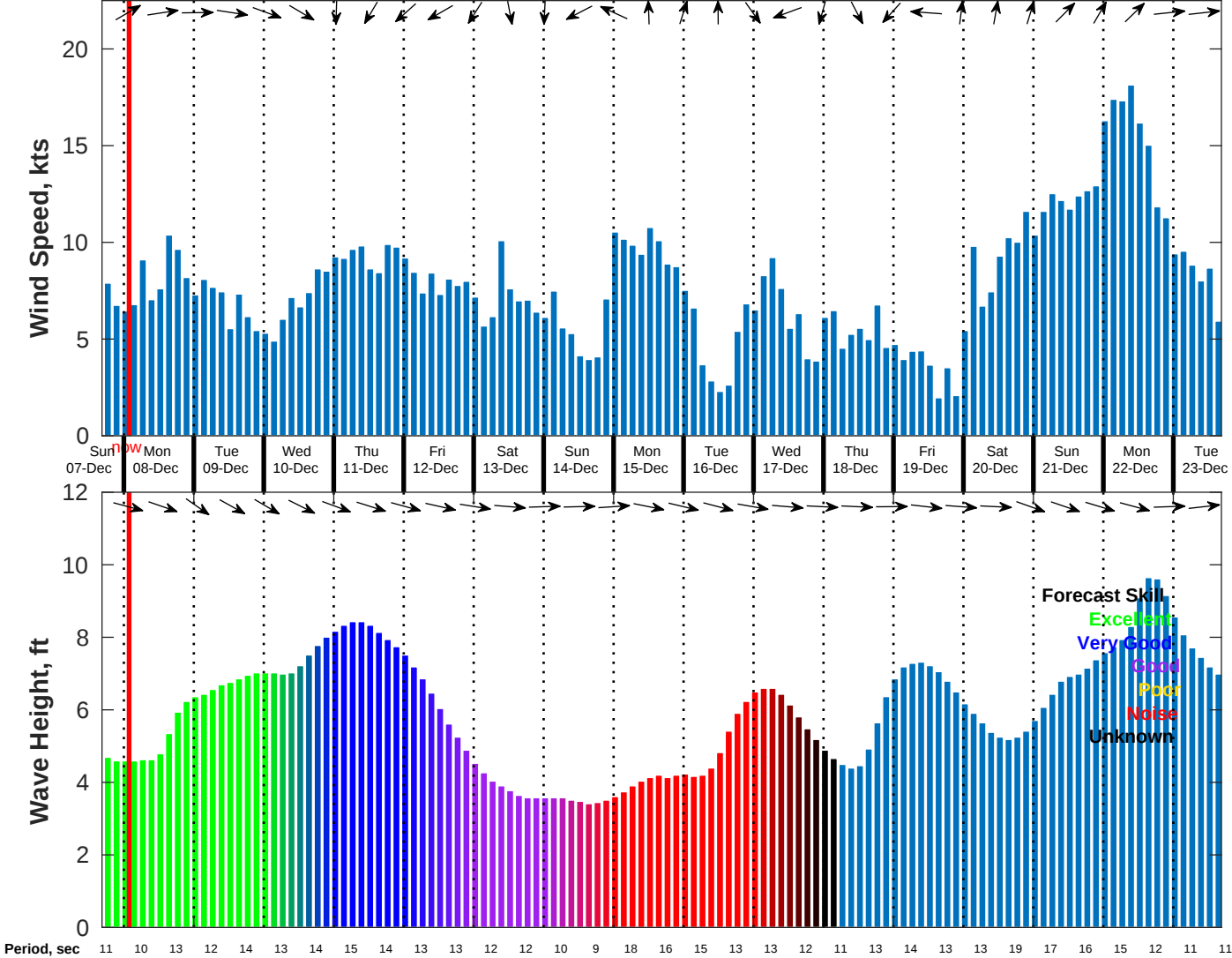
Wind & Wave Forecast for NDBC 46059 from 07-Dec-2025 17:00:00 to 23-Dec-2025 17:00:00
