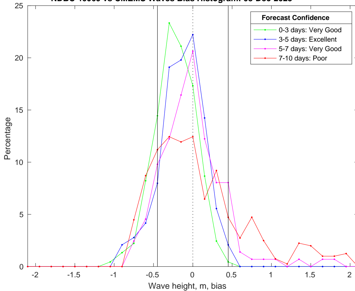
NDBC 46069 vs CMEMS Waves Bias Histogram: 08-Dec-2025
