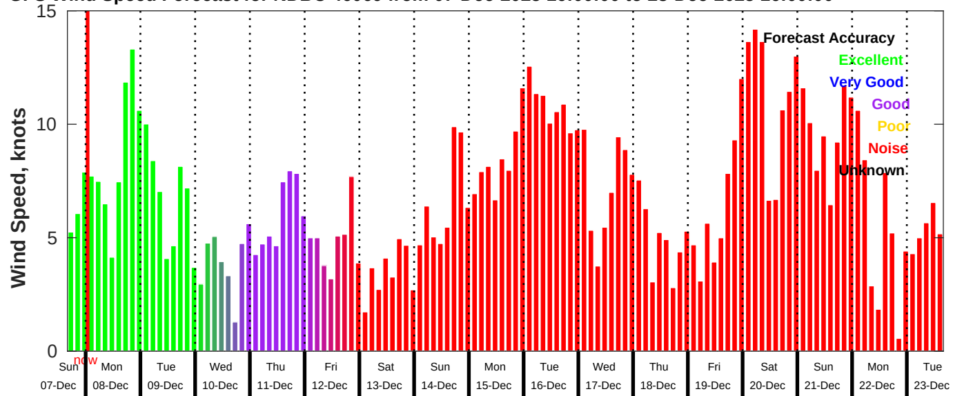
GFS Wind Speed Forecast for NDBC 46069 from 07-Dec-2025 16:00:00 to 23-Dec-2025 16:00:00
