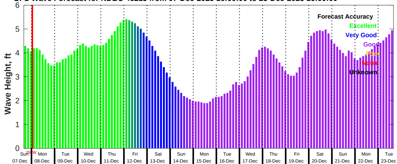
GFS Wave Forecast for NDBC 46215 from 07-Dec-2025 16:00:00 to 23-Dec-2025 16:00:00
