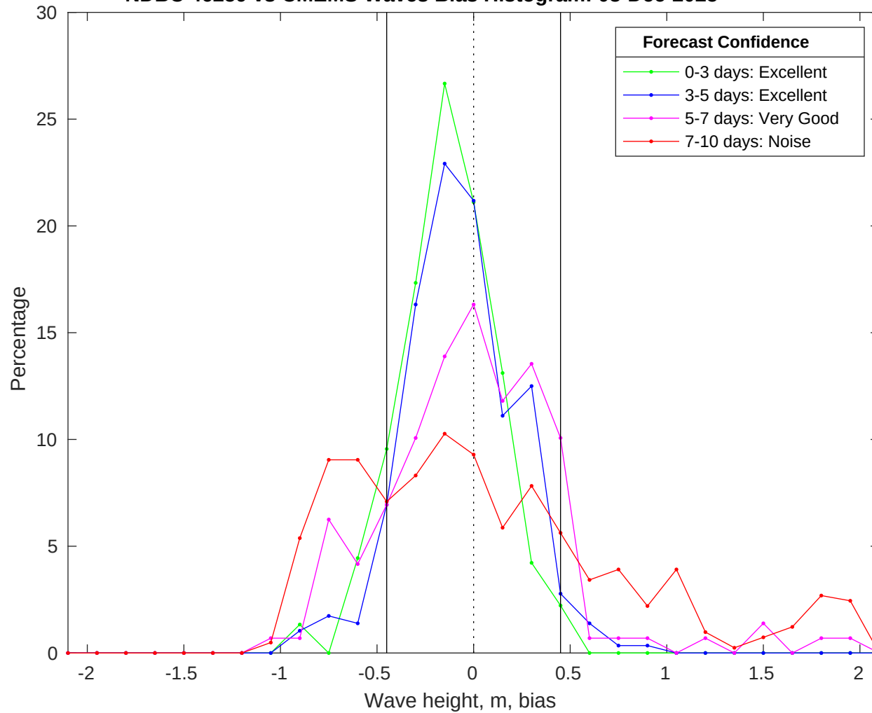
NDBC 46259 vs CMEMS Waves Bias Histogram: 08-Dec-2025
