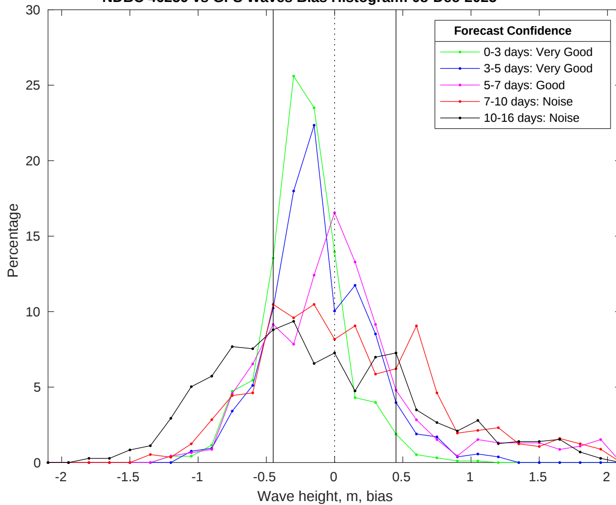
NDBC 46259 vs GFS Waves Bias Histogram: 08-Dec-2025
