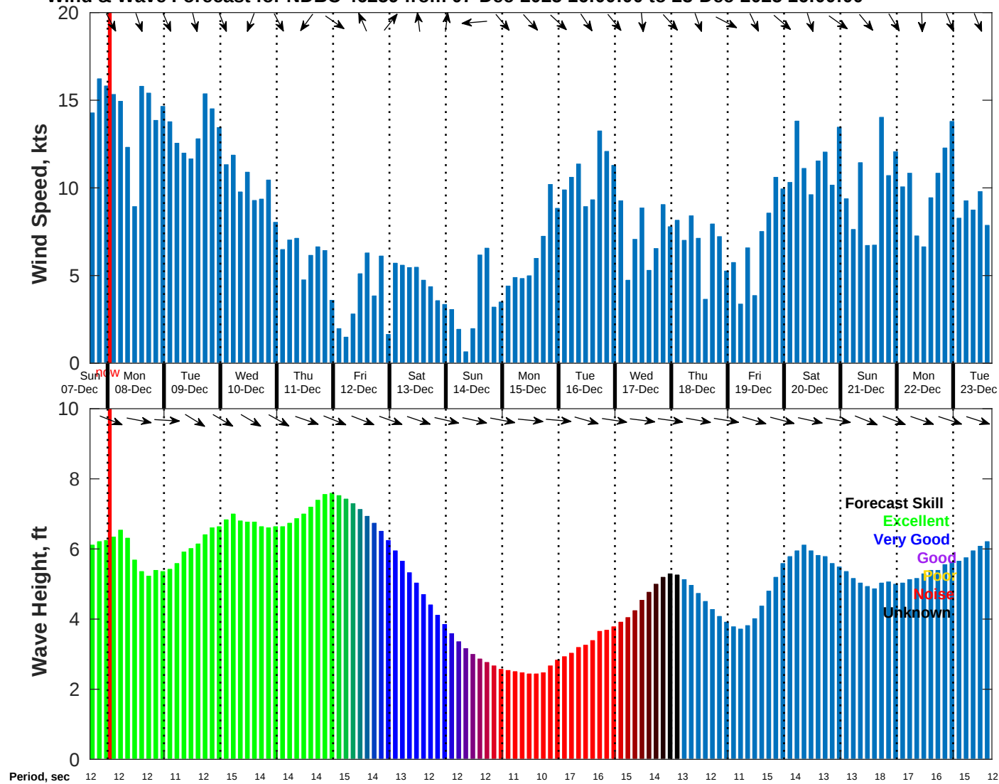
Wind & Wave Forecast for NDBC 46259 from 07-Dec-2025 16:00:00 to 23-Dec-2025 16:00:00
