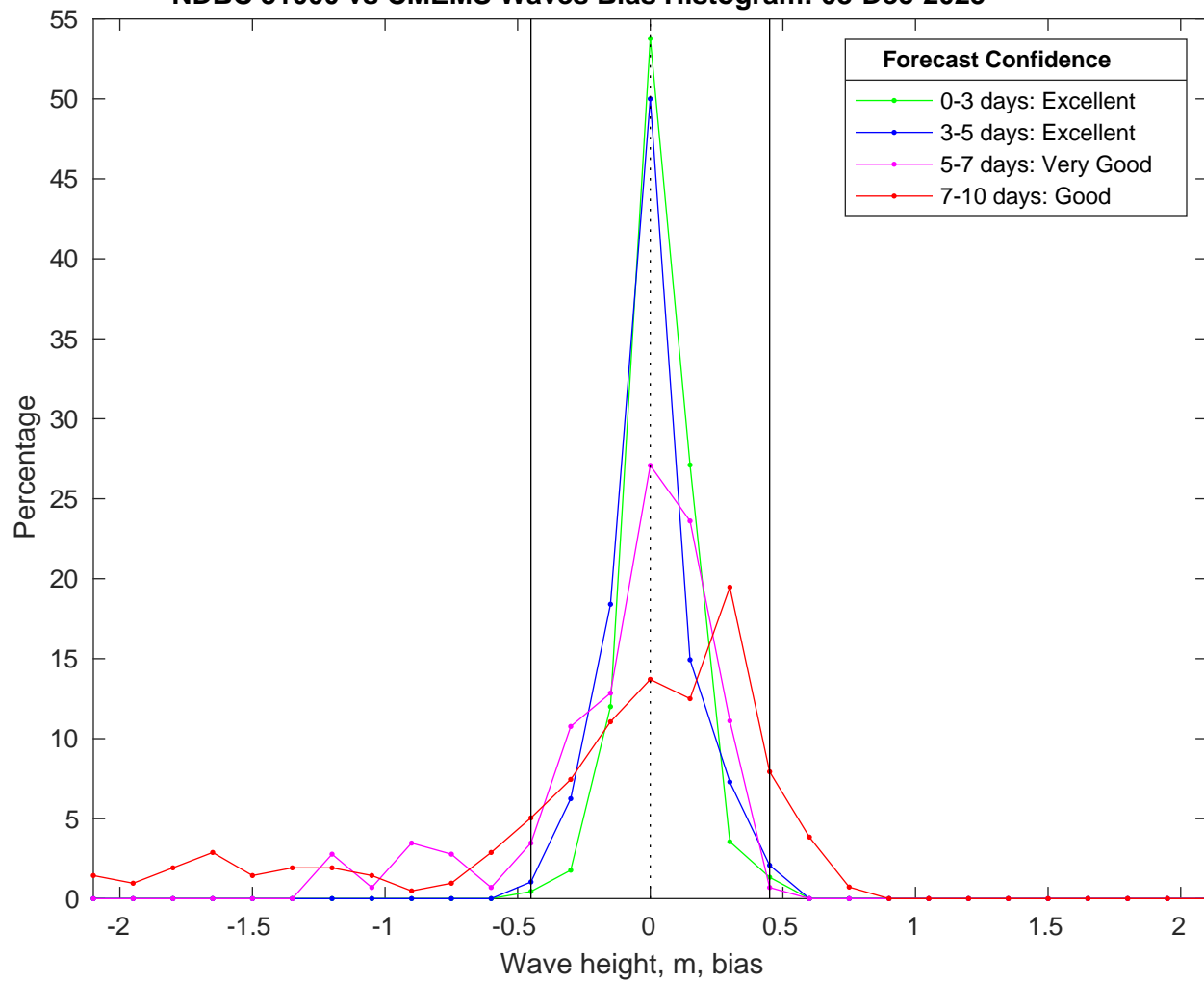
NDBC 51000 vs CMEMS Waves Bias Histogram: 08-Dec-2025
