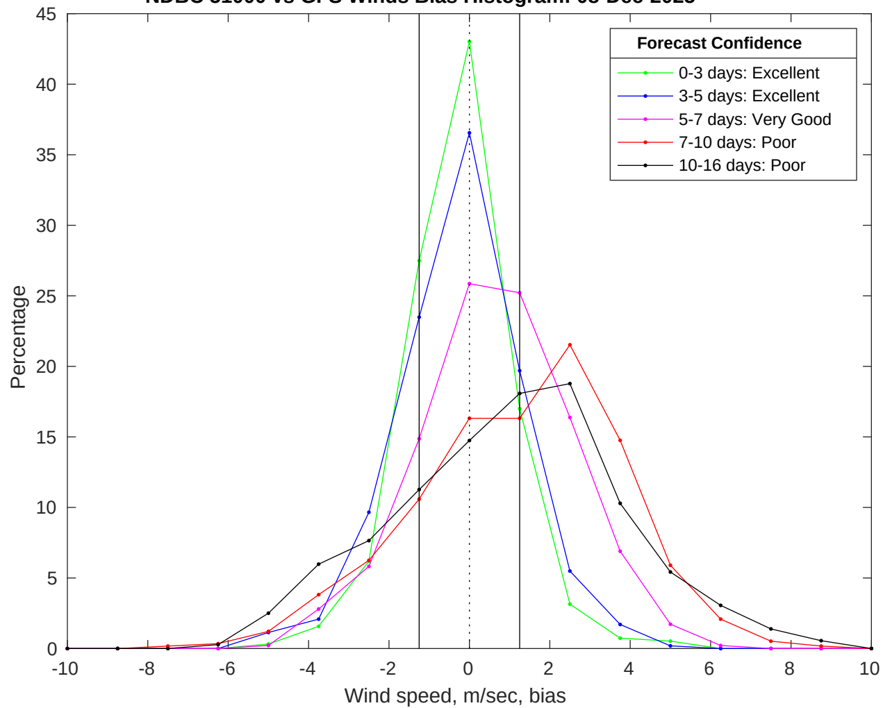
NDBC 51000 vs GFS Winds Bias Histogram: 08-Dec-2025
