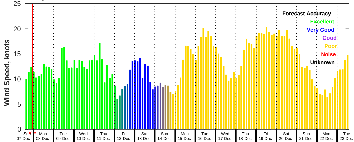
GFS Wind Speed Forecast for NDBC 51000 from 07-Dec-2025 14:00:00 to 23-Dec-2025 14:00:00
