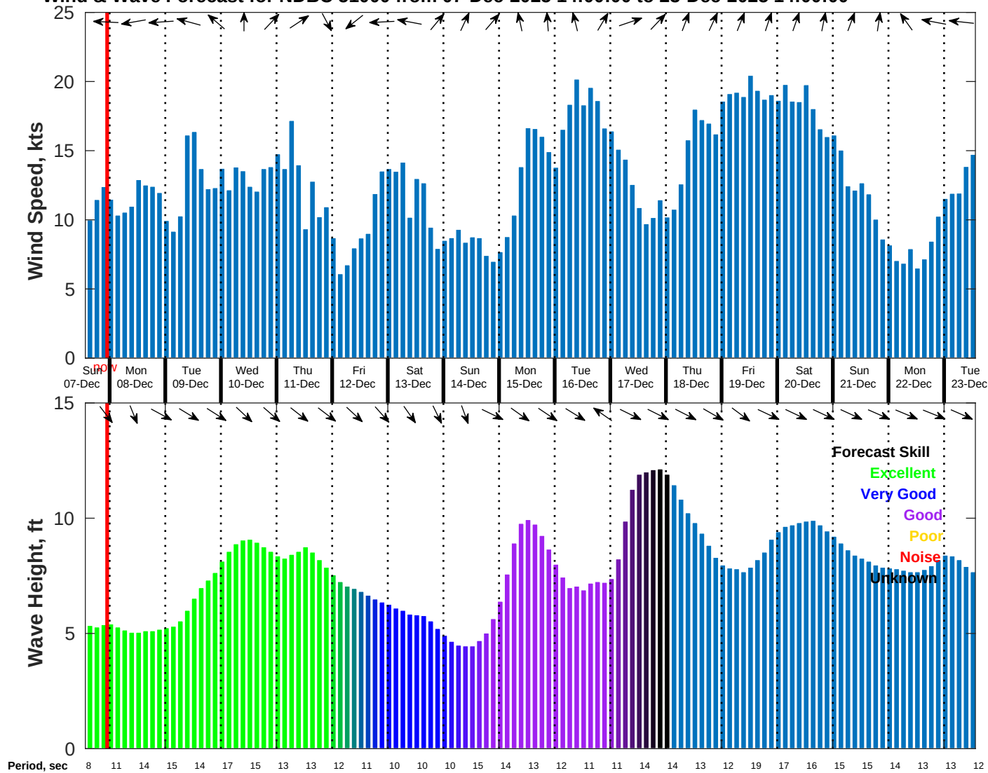
Wind & Wave Forecast for NDBC 51000 from 07-Dec-2025 14:00:00 to 23-Dec-2025 14:00:00
