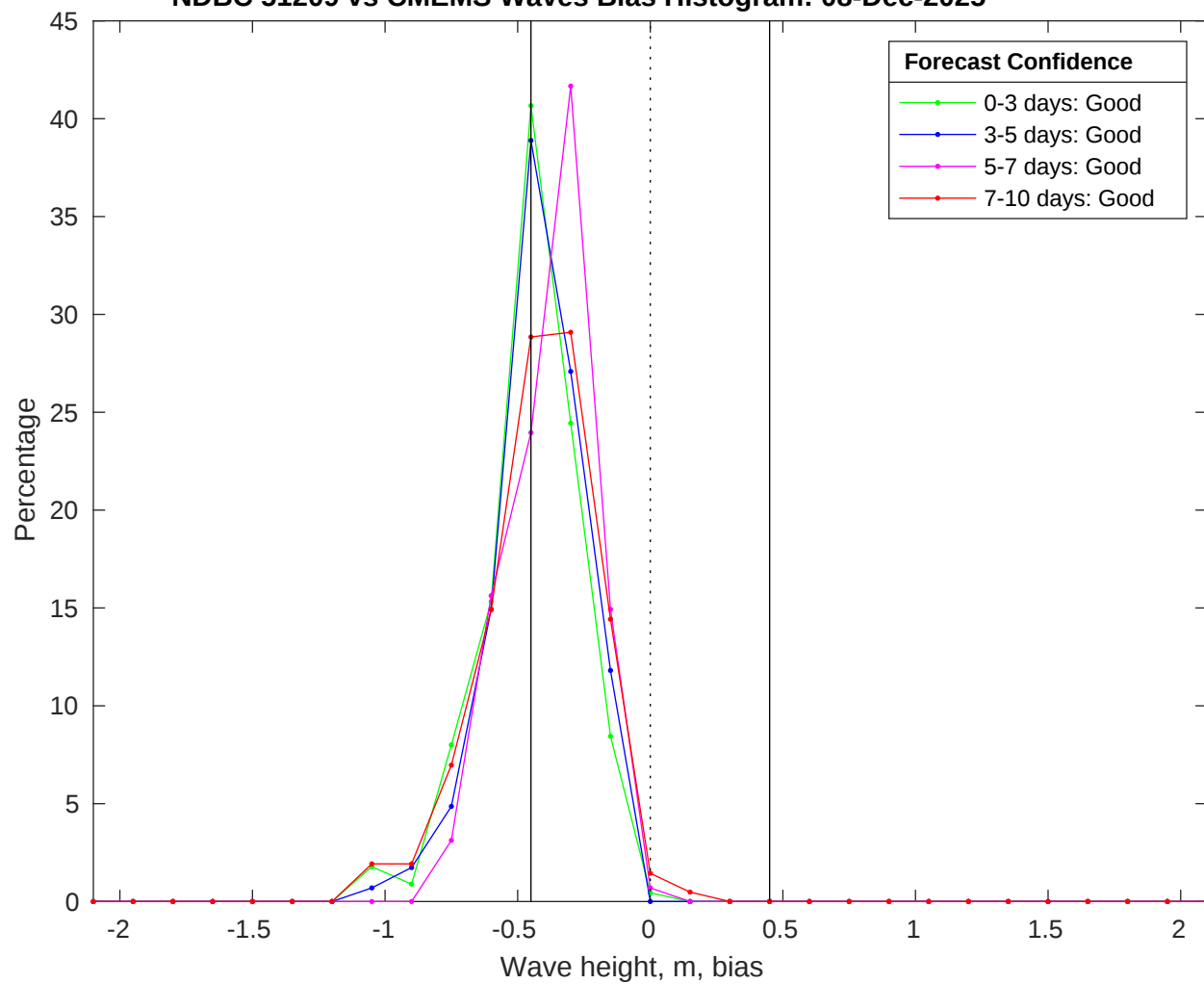
NDBC 51209 vs CMEMS Waves Bias Histogram: 08-Dec-2025
