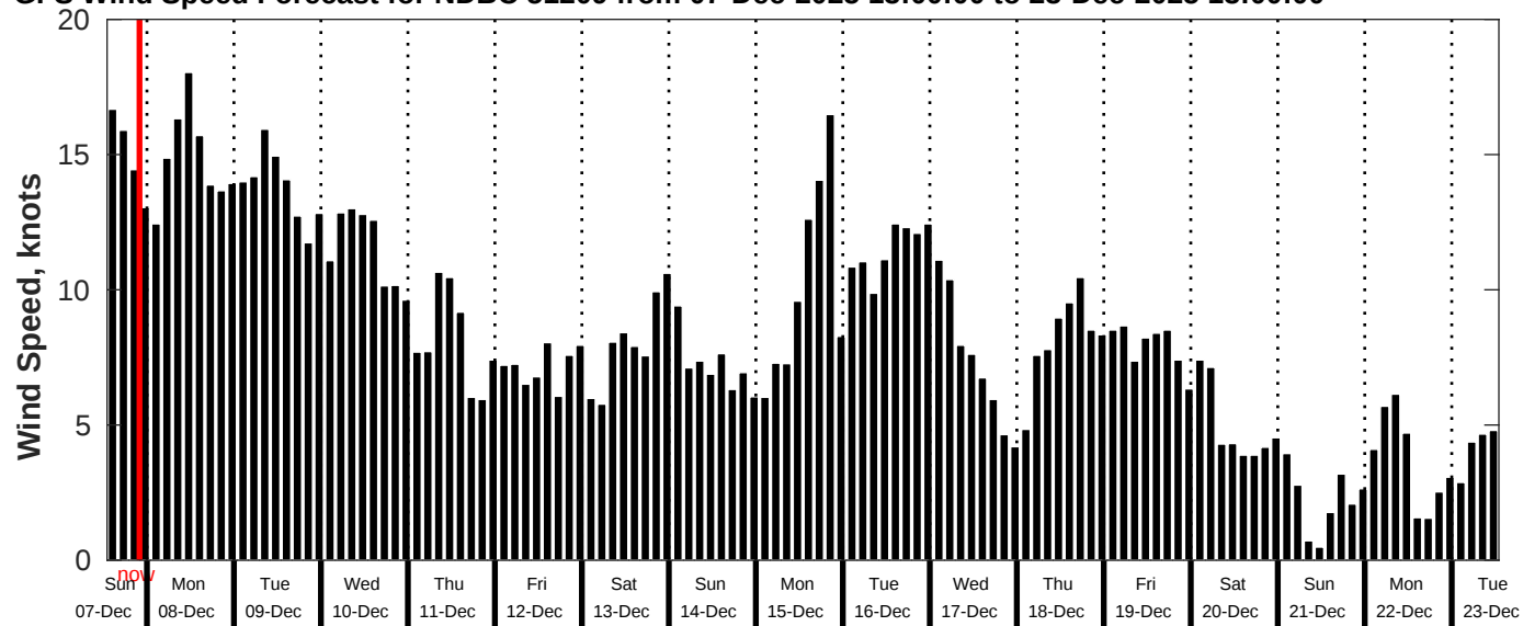
GFS Wind Speed Forecast for NDBC 51209 from 07-Dec-2025 13:00:00 to 23-Dec-2025 13:00:00
