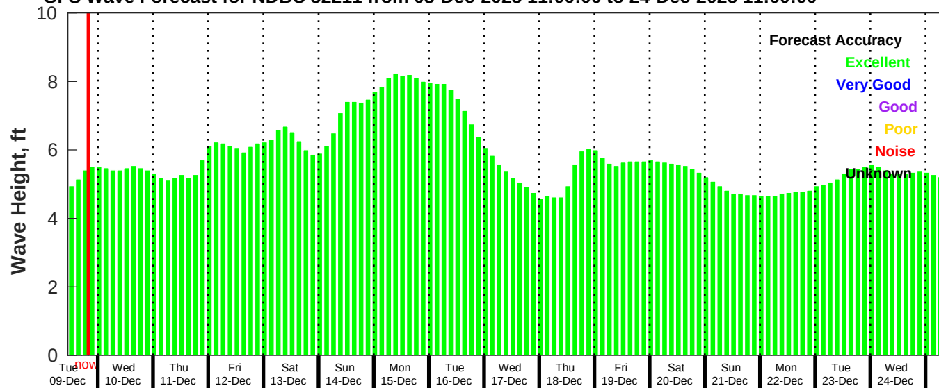
GFS Wave Forecast for NDBC 52211 from 08-Dec-2025 11:00:00 to 24-Dec-2025 11:00:00
