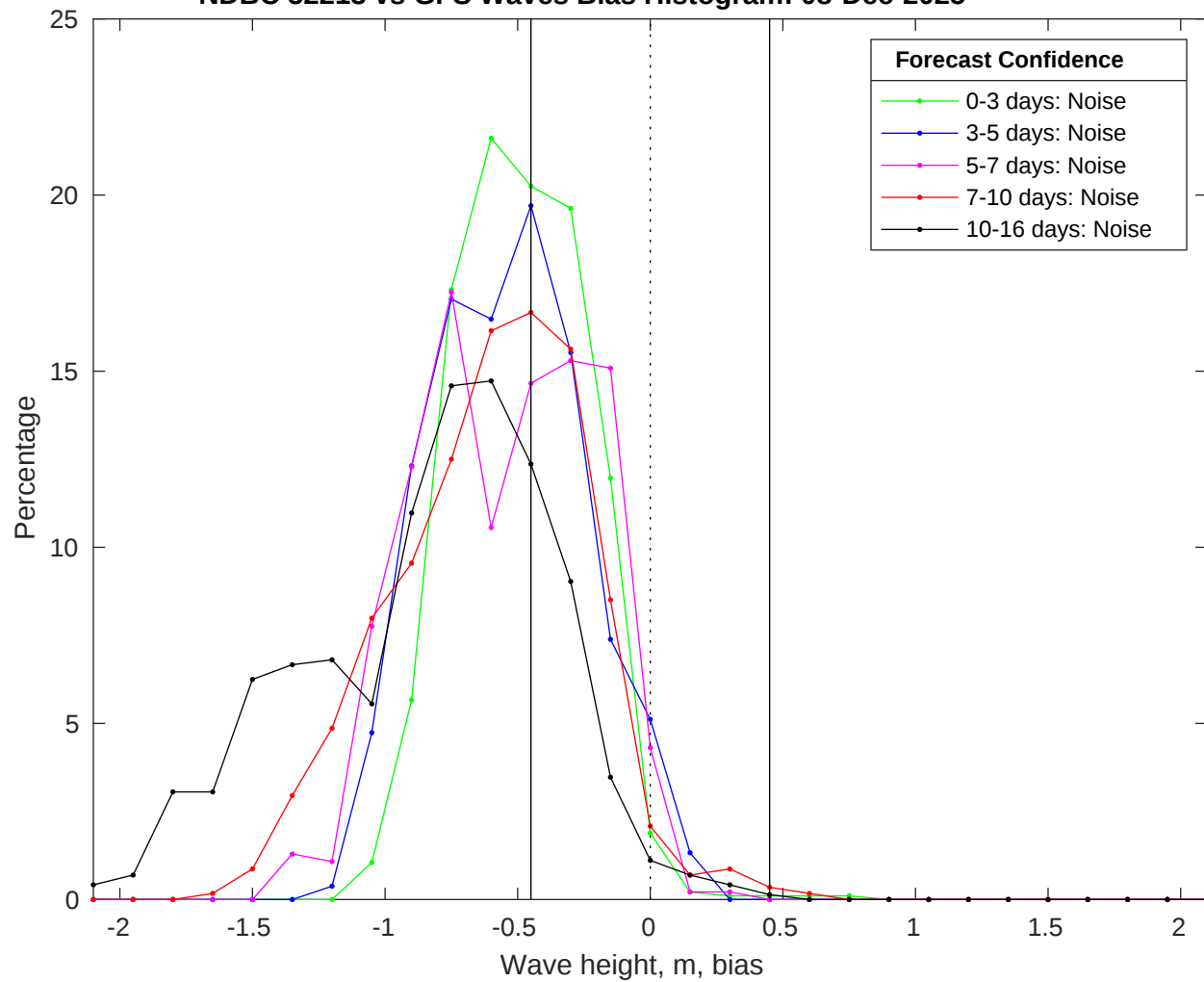
NDBC 52213 vs GFS Waves Bias Histogram: 08-Dec-2025
