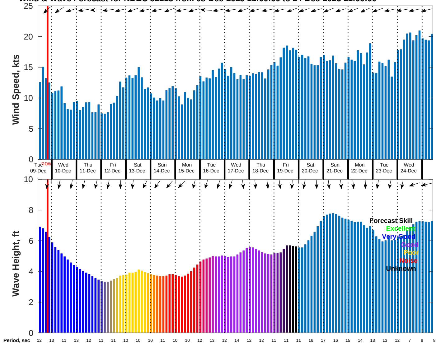
Wind & Wave Forecast for NDBC 52213 from 08-Dec-2025 11:00:00 to 24-Dec-2025 11:00:00
