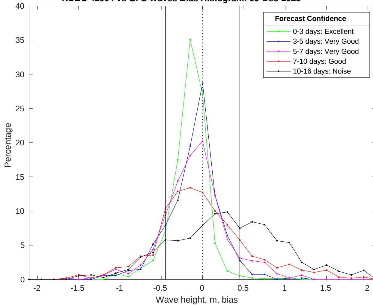
NDBC 41004 vs GFS Waves Bias Histogram: 09-Dec-2025
