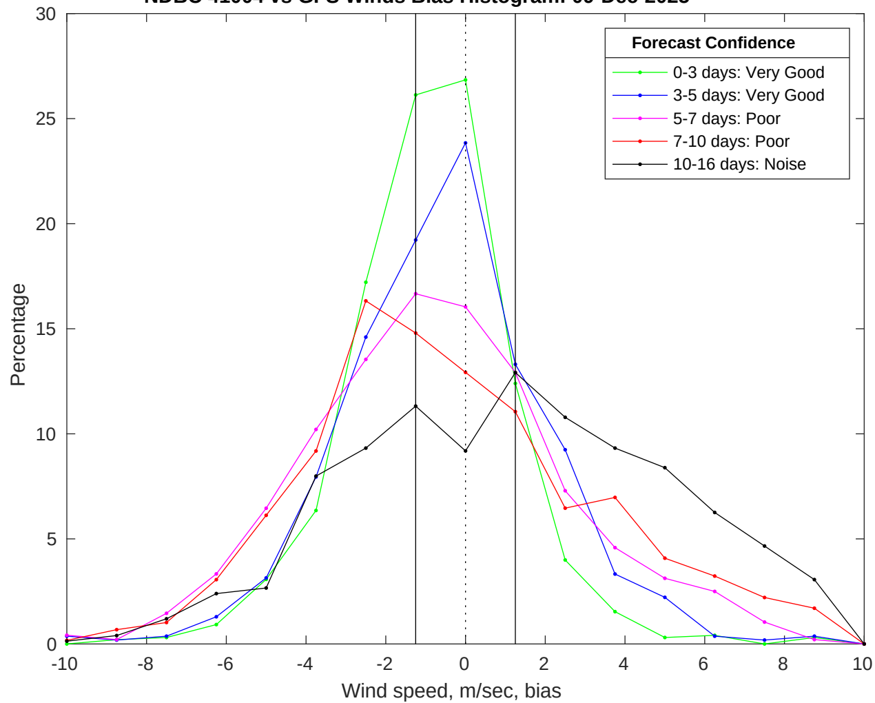
NDBC 41004 vs GFS Winds Bias Histogram: 09-Dec-2025
