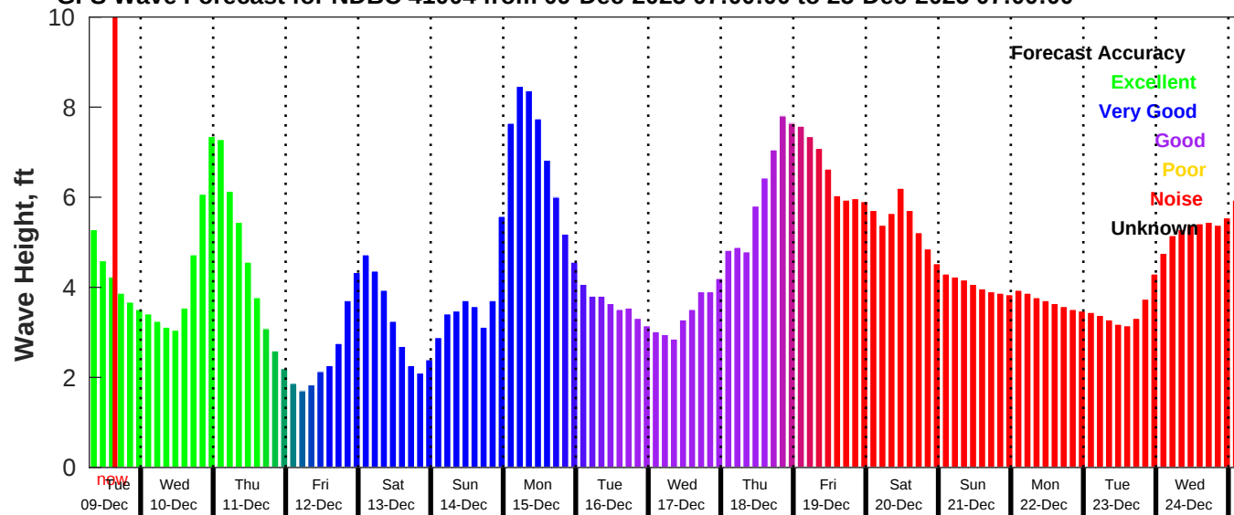
GFS Wave Forecast for NDBC 41004 from 09-Dec-2025 07:00:00 to 25-Dec-2025 07:00:00
