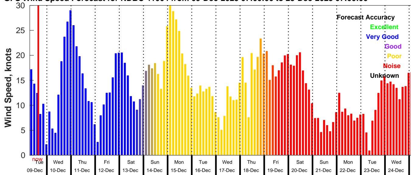
GFS Wind Speed Forecast for NDBC 41004 from 09-Dec-2025 07:00:00 to 25-Dec-2025 07:00:00
